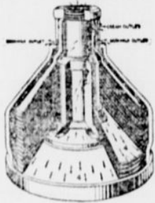
Cross-section of new bowl, showing new method of distributing milk between the discs.
